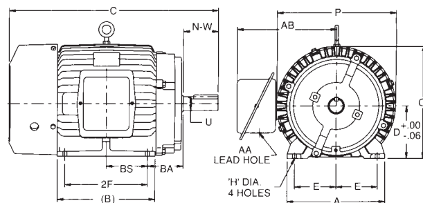
Typical Rigid Base Motor
