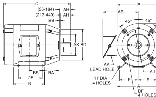
Typical C-Face Motor
